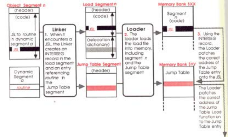
Figure 15-5A How the Jump Table works
