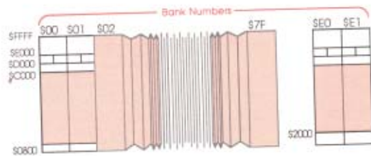
Figure 3-4 Memory allocatable through the Memory Manager
