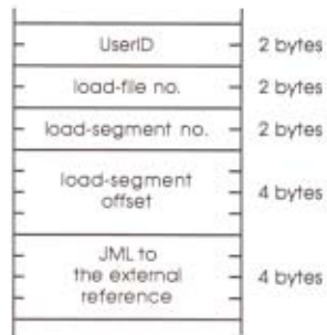
Figure 15-4 Jump Table entry (loaded state)
