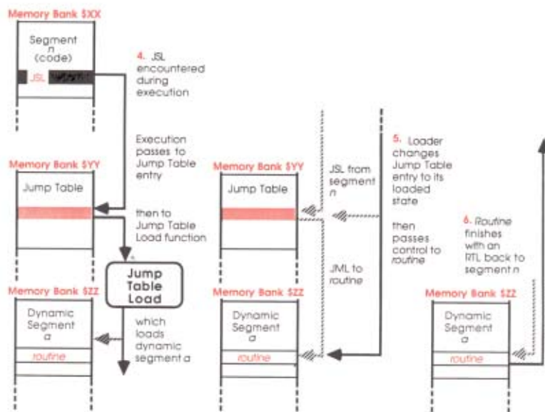
Figure 15-5B How the Jump Table works (continued)
