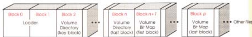
Figure A-1 Block organization of a volume
