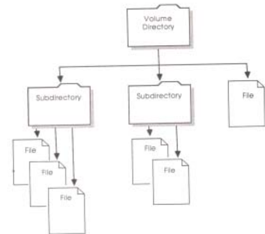
Figure 1-2 Example of a hierarchical file structure
