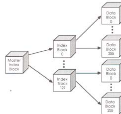
Figure 2-5 Block organization of a standard file
