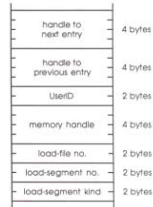
Figure 15-1 Memory Segment Table entry
