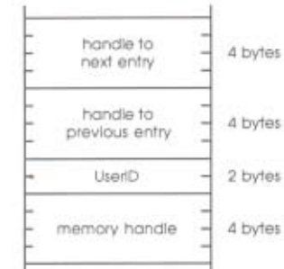
Figure 15-2 Jump Table Directory entry
