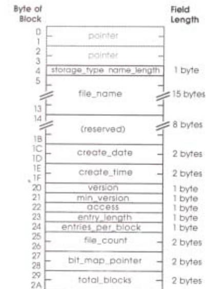
Figure A-3 The volume directory header
